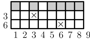
FIGURE 4. The resulting grid for L = \{1, 2, 3, 4, 5, 6, 7, 8\} .
